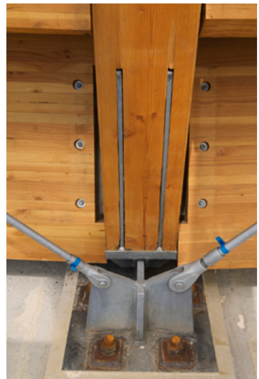
Double kerf plates and hidden 1" steel pins were used to connect the ribs and mullions. These intricate connections were shop fabricated for ease of construction. © John Blaustein 2008.
